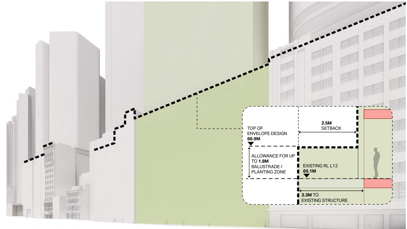
Proposed Envelope Close-up - Castlereagh Street, looking south.
